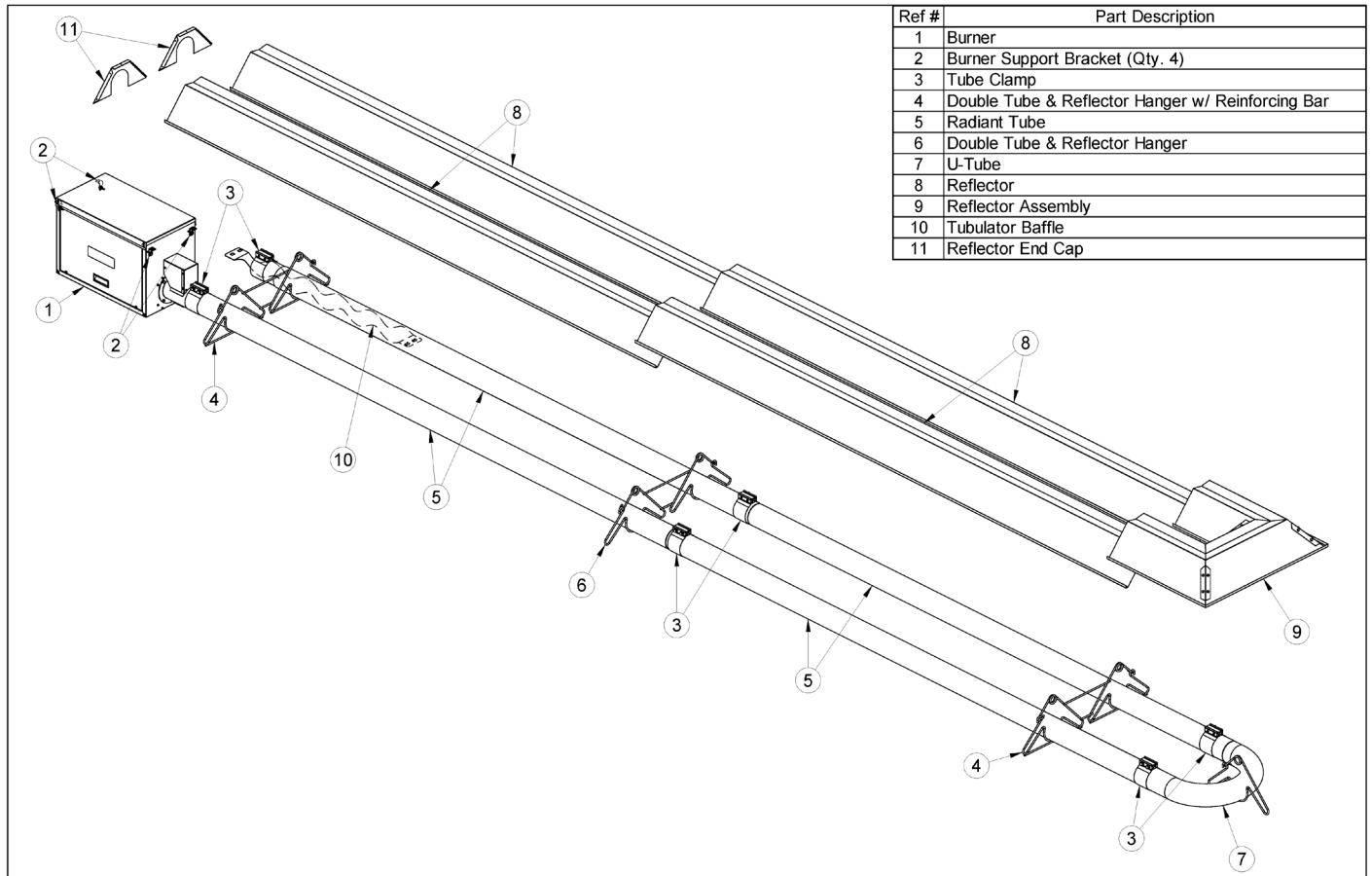
Figure 7.1 - U-Tube System Components
