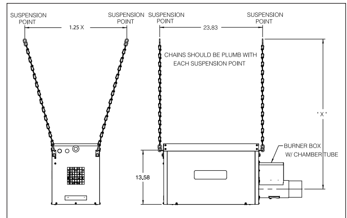
Figure 10.4 - Burner Suspension
