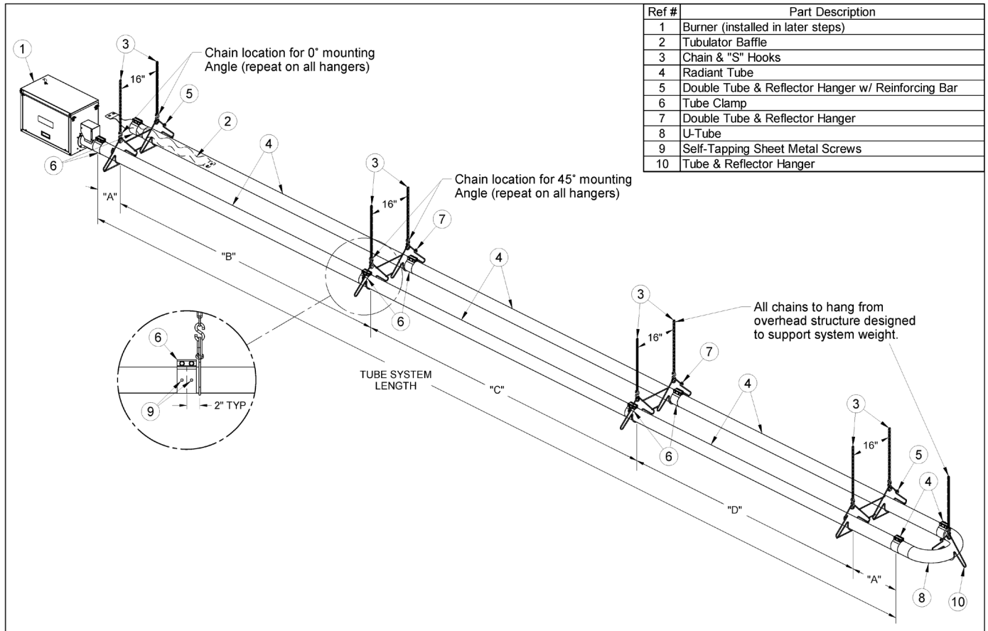
Figure 9.1 - U-Tube System Suspension
