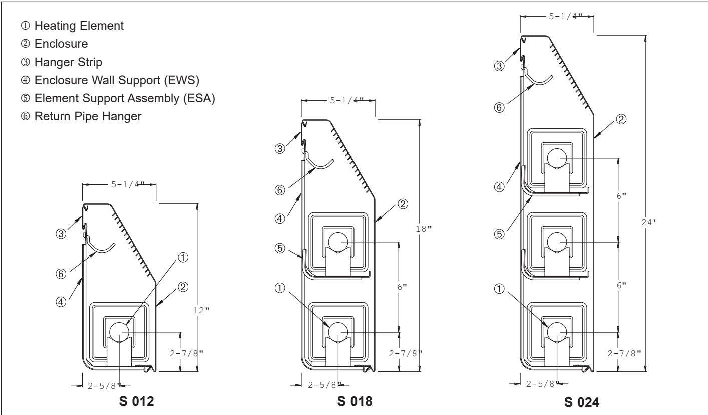
Figure 14.1 - System Components
