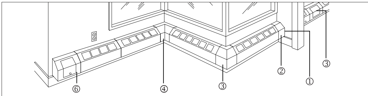
Figure 5.4 - Typical Enclosure Layout
