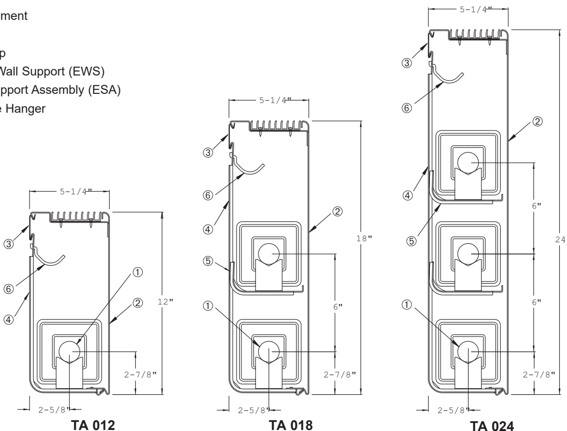
Figure 28.1 - System Components
