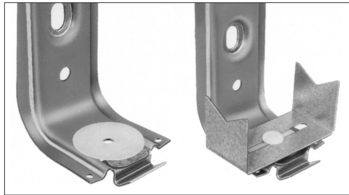
Figure 4.4 - Bottom Enclosure Support
