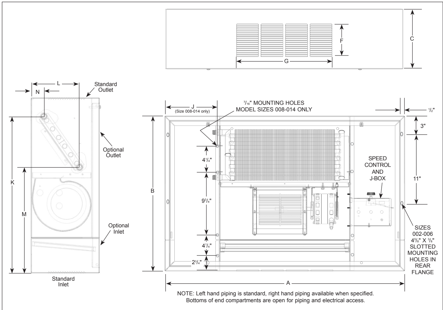
Figure 15 - Wall or Ceiling Model CW, Sizes 002-014 Steam/Hot Water Cabinet Unit Heaters ①
