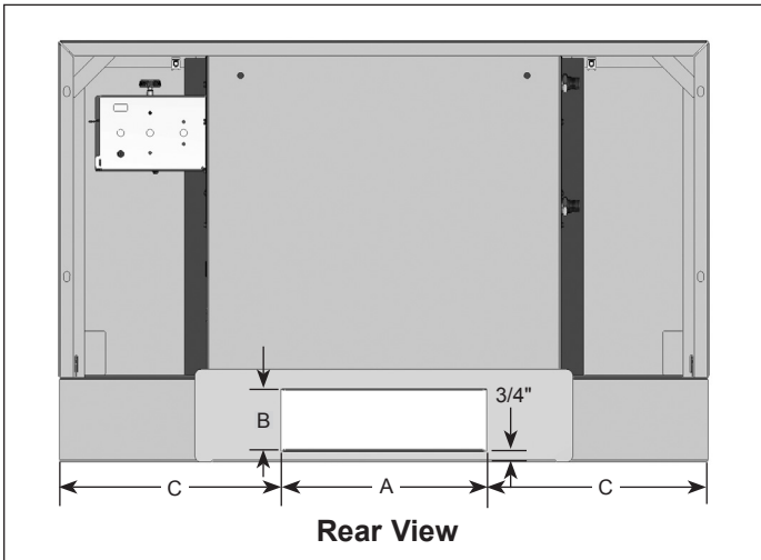
Figure 18 - Model C - Outside Air Duct Collar
