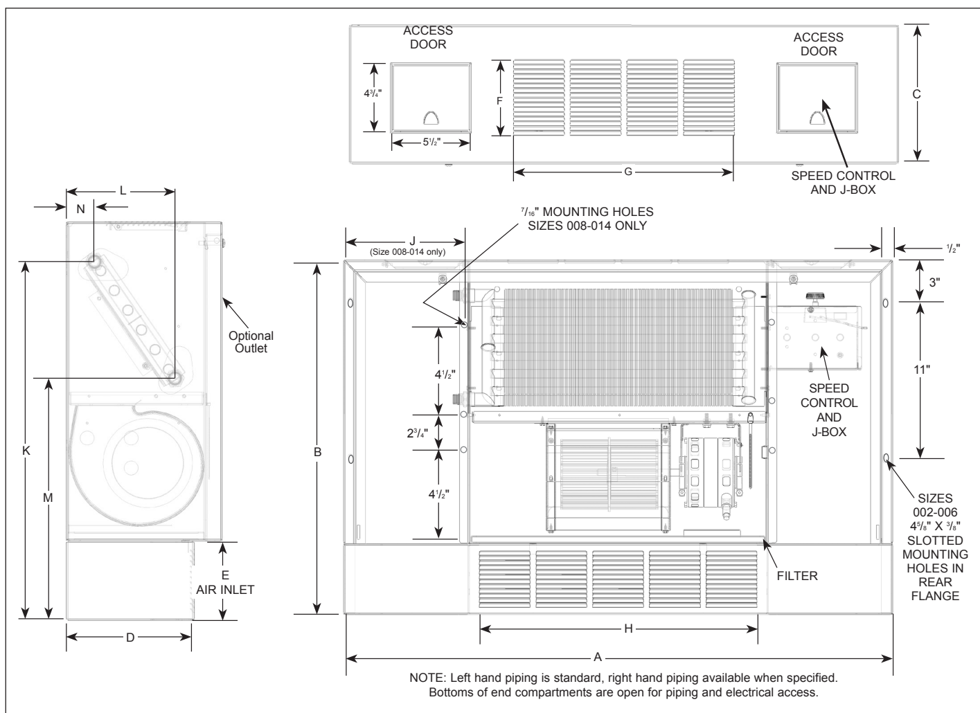
Figure 14 - Floor Model C, Sizes 002-014 Steam/Hot Water Cabinet Unit Heaters
