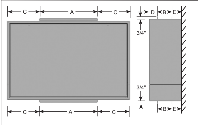
Figure 17 - Model CW - Duct Collars
