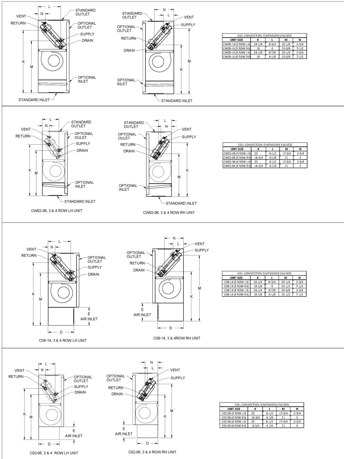
Figure 16 - C & CW Coil Connections Dimensions (3 & 4 Row Coil Units):
