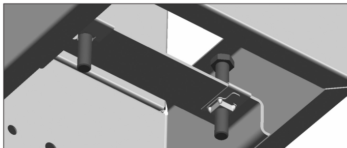
Figure 9 - Leveling Bolts
