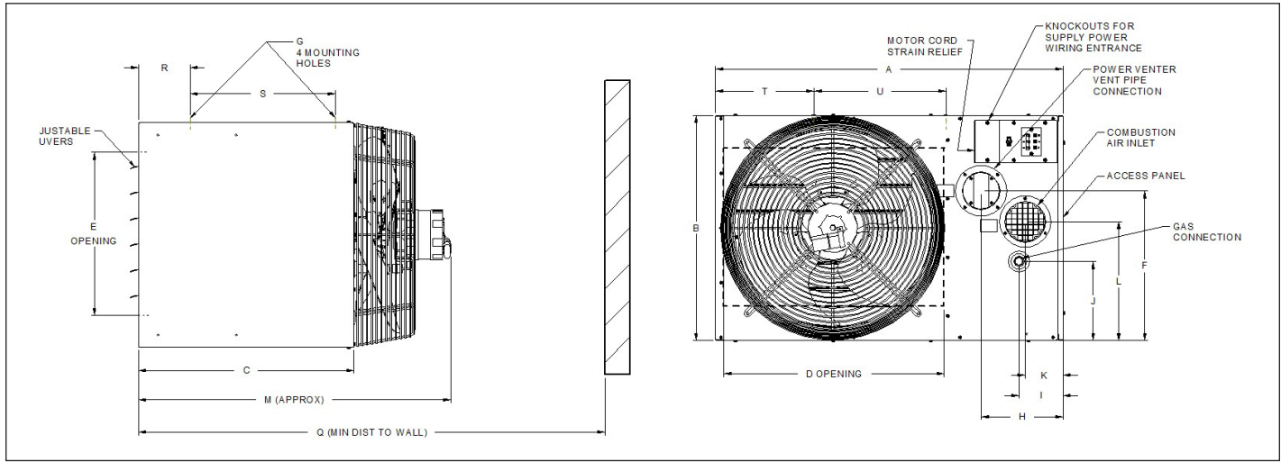
Figure 24.1 - Dimensional Drawings
